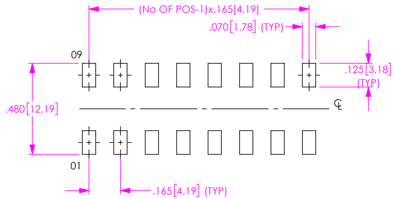
-DV LAYOUT SHOWN FOR IPBS-108-X2-X-D
