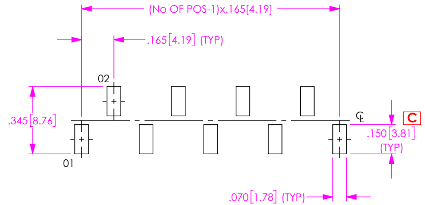
-SV *NOT RELEASED FOR PRODUCTION LAYOUT SHOWN FOR IPBS-109-X2-X-S
